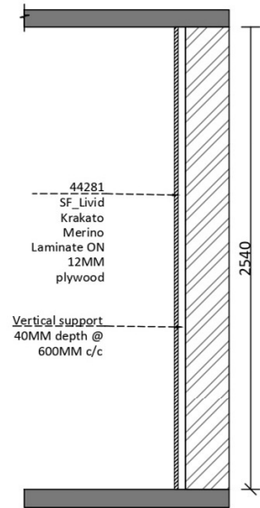
TYPICAL WALL SECTION DETAIL SCALE:1:25
