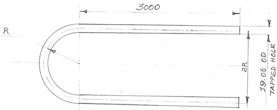
DETAIL OF "U" TUBE
