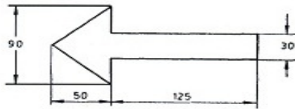
6B For Pipes Above DN 200 SIZE OF ARROWS
